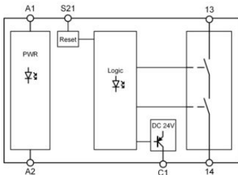
Abb. 1 Block Diagram SD1K
