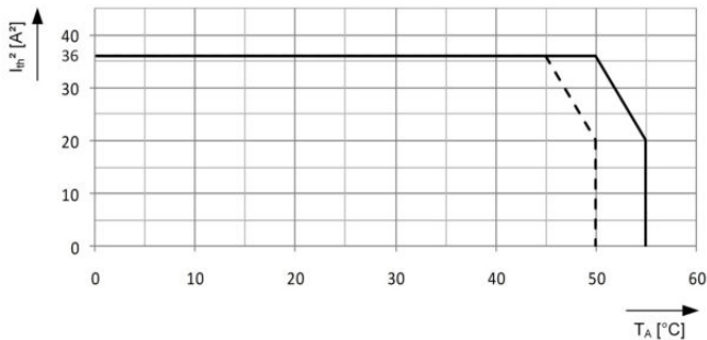
Fig. 11 Deratingkurve
