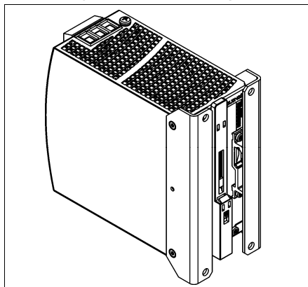
Fig. 24-1 Wall mounting
