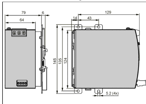
Fig. 24-5 Mounting Dimensions Side mounting bracket
