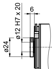
BHF/BHG Klemmring
