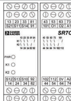
Abb. 3 Anschlüsse
