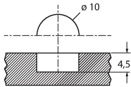
Drawing R10-M
