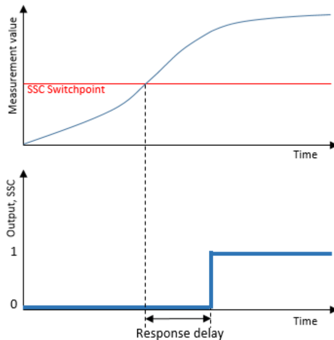
Figure 18: Response Delay
