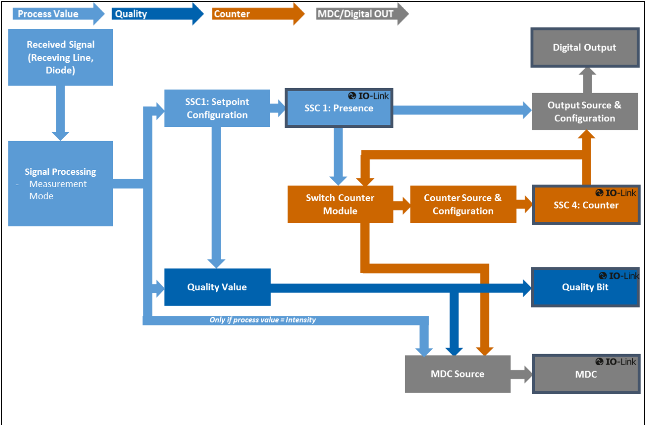
Figure 3 Illustrates the signal path from raw data to an output either through a physical pin (top right) or as output via the process data (bottom right)
