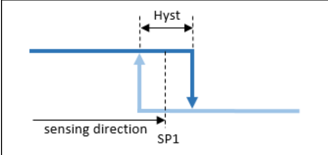
Figure 16 Center Aligned, Single Point Mode
