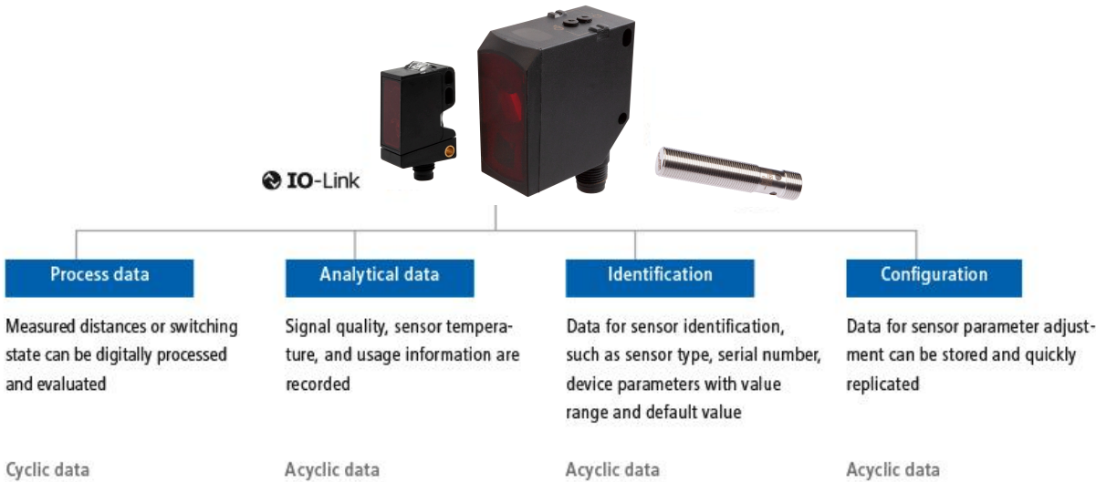
Figure 2 Different IO Link data streams
