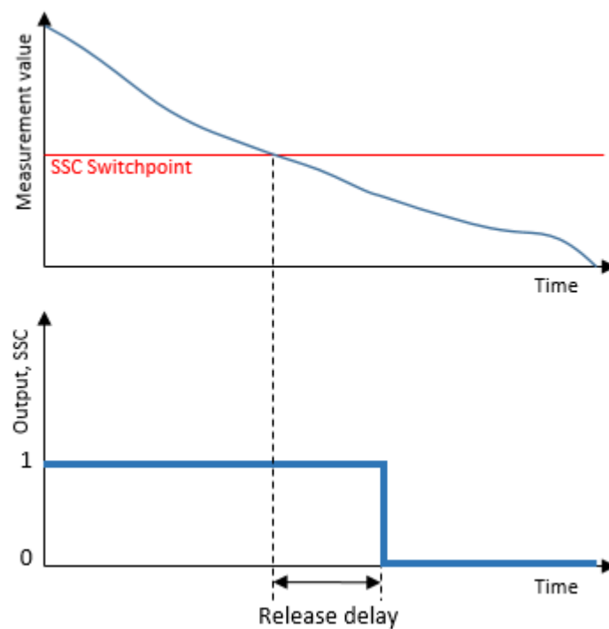
Figure 19: Release Delay
