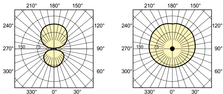
LDLD_MHN-TD-Light distribution diagram
