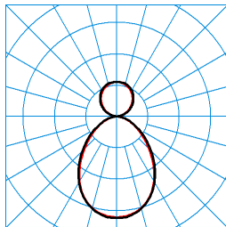
SFlow H2-L MRWD LED6400-830 01 TX372632
