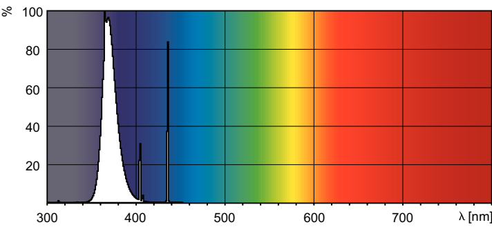
Spectral Power Distribution Colour - TL 100W/10-R UV-A
