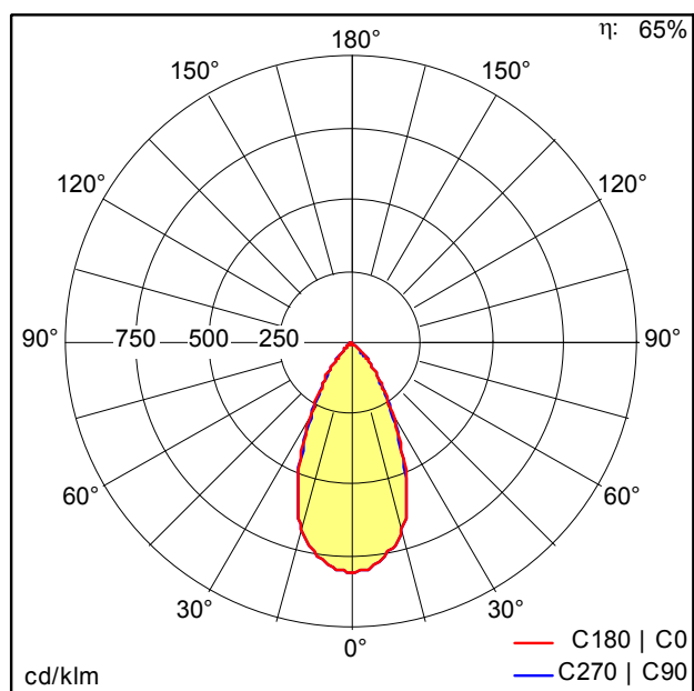
ST7745_M.Idt
