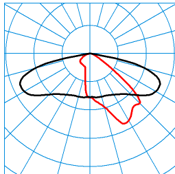
US 9701-AB2L-LR/220/260/320-740 4G1 (2600 lm) TX055655
