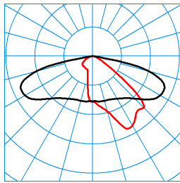
US 9701-AB2L-LR/220/260/320-740 4G1 (2200 lm) TX055654
