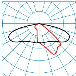
US 9701-AB2L-LR/220/260/320-740 4G1 (3200 lm) TX055675
