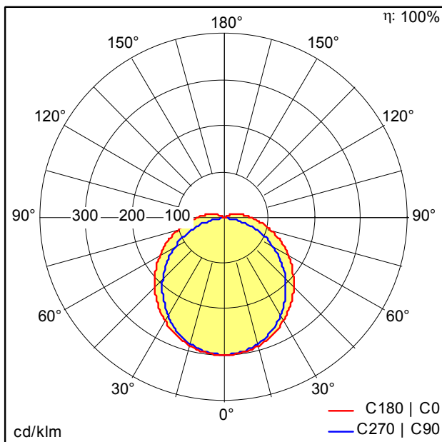
TE_JULIE_1500_LED_IP65_6300_840_TW.Idt
