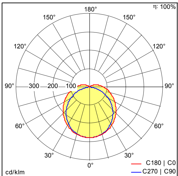
TE_LUCY_1800_LED_IP66_8000_840_TW.ltd
