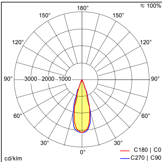
TE_LILY_LED_SPOT_IP44_24_68_850_930.idt
