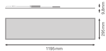
Product line drawing with numbers
