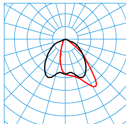
Jovie 70I-AM3L-MLLR/56-68-730 8G1 ETDD (CLO initial value) TX264166 DIN 5040: A50 UTE: 1,00 D CEN Flux Code: 59 89 100 100 100 ■ C0 - C180 ■ C90 - C270
