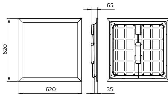
RC066B LED34S/840 PSD W62L62 OC
