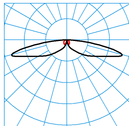
CS 19 100-SB3L-SLR1/5100-740 4G1S ET (CLO initial value) TX300162 DIN 5040: A20 UTE: 1,00 J CEN Flux Code: 23 53 85 100 100 0 0 0 0 ■ C0 - C180 ■ C90 - C270
