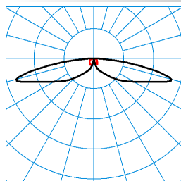
CS 19 100-SB3L-SLR1/5100-740 4G1S ET (CLO end value) TX300161 DIN 5040: A20 UTE: 1,00 J CEN Flux Code: 23 53 85 100 100 0 0 0 0 ■ C0 - C180 ■ C90 - C270
