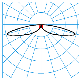
CS 19 100-SB3L-SLR1/2200-740 2G1S ET (CLO initial value) TX300158 DIN 5040: A20 UTE: 1,00 J CEN Flux Code: 22 52 84 100 100 0 0 0 0 ■ C0 - C180 ■ C90 - C270
