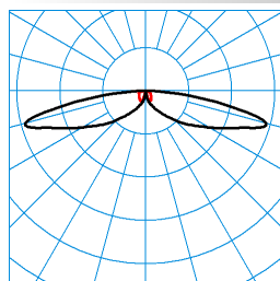
CS 19 100-SB3L-SLR1/2200-740 2G1S ET (CLO end value) TX300157 DIN 5040: A20 UTE: 1,00 J CEN Flux Code: 22 52 84 100 100 0 0 0 0 ■ C0 - C180 ■ C90 - C270
