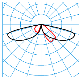
CS 19 100-AB2L/1200-730 2G1S ETDD (CLO initial value) TX299963 ■ C0 - C180 ■ C90 - C270 DIN 5040: A20 UTE: 1,00 l CEN Flux Code: 26 63 96 100 100
