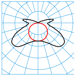
AragF 12 P-XW 23-840 +DMM PC TX281220
