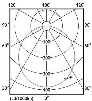
Downlight DN065C G3 LDNR CCT D200 RD-LDD
