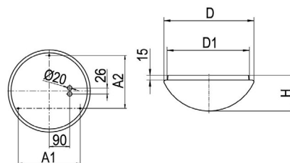
Maße [mm]
