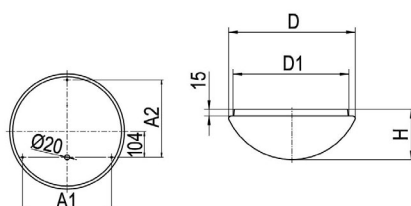
Maße [mm]
