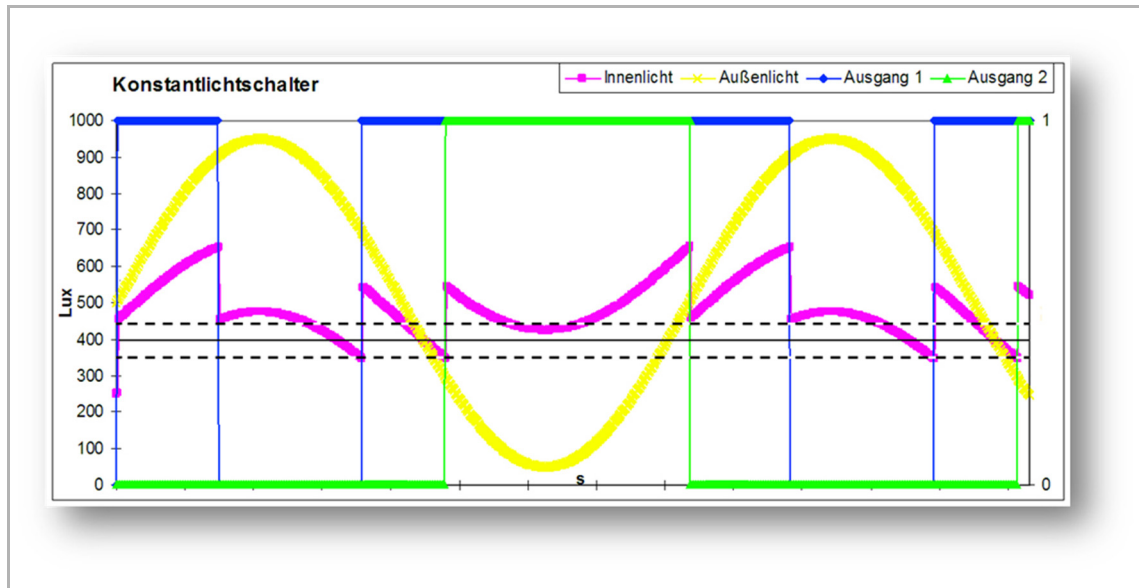
Fig. 22: Time sequence of the constant light switch.
