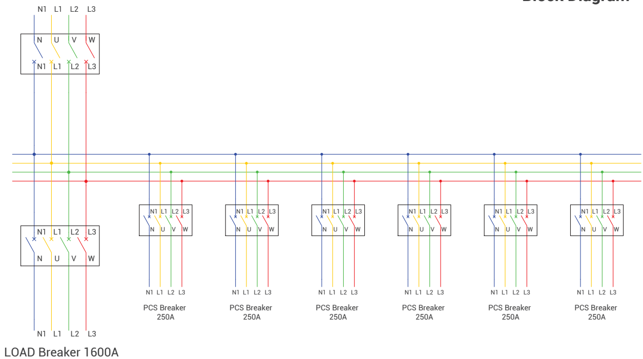
GRID Breaker 1600A
